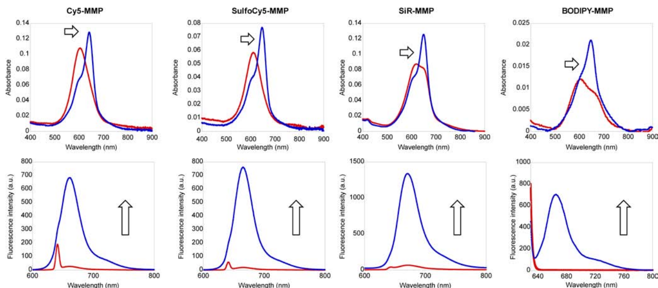
Figure 3. (Top) Absorption spectra before (red) and after enzymatic reaction (blue) of the four MMP probes, Cy5-MMP ( 1 \mu\text{M} ), SulfoCy5-MMP ( 1 \mu\text{M} ), SiR-MMP ( 1 \mu\text{M} ), BODIPY-MMP ( 2 \mu\text{M} ) in 1 mL TCN buffer containing 0.1% DMSO (for Cy5-MMP , SulfoCy5-MMP , and SiR-MMP ) or 3% DMSO (for BODIPY-MMP ) as a cosolvent. (bottom) Fluorescence spectra of the MMP probes, Cy5-MMP ( 1 \mu\text{M} ), SulfoCy5-MMP ( 1 \mu\text{M} ), SiR-MMP ( 1 \mu\text{M} ), BODIPY-MMP ( 2 \mu\text{M} ), incubated with 1 \mu\text{g} of MMP2 (catalytic domain recombinant protein) in 1 mL TCN buffer containing 0.1% DMSO (for Cy5-MMP , SulfoCy5-MMP , and SiR-MMP ) or 3% DMSO (for BODIPY-MMP ) as a cosolvent at 37^\circ\text{C} for 300 min ( Cy5-MMP ), 840 min ( SulfoCy5-MMP ), 600 min ( SiR-MMP ), or 240 min ( BODIPY-MMP ) with excitation at 620 nm (for BODIPY-MMP ) or 640 nm (for Cy5-MMP , SulfoCy5-MMP , and SiR-MMP ). Spectra were measured before (red) and after (blue) enzymatic reaction.
