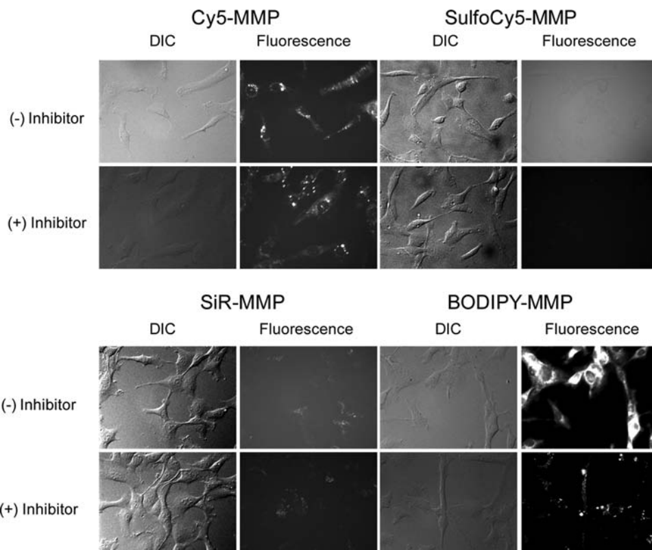
Figure 4. Bright field and fluorescence images of HT-1080 cells incubated with Cy5-MMP , SulfoCy5-MMP , SiR-MMP , or BODIPY-MMP ( 1 \mu\text{M} , final 0.2% DMSO as a cosolvent) at 37^\circ\text{C} for 3 h in the presence (bottom) or the absence (top) of the inhibitor GM6001 ( 100 \mu\text{M} ).
